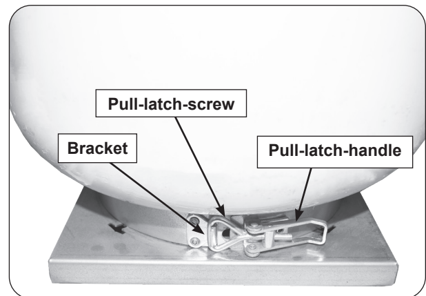
Fig. 28-3 Secure L.P. cylinder
