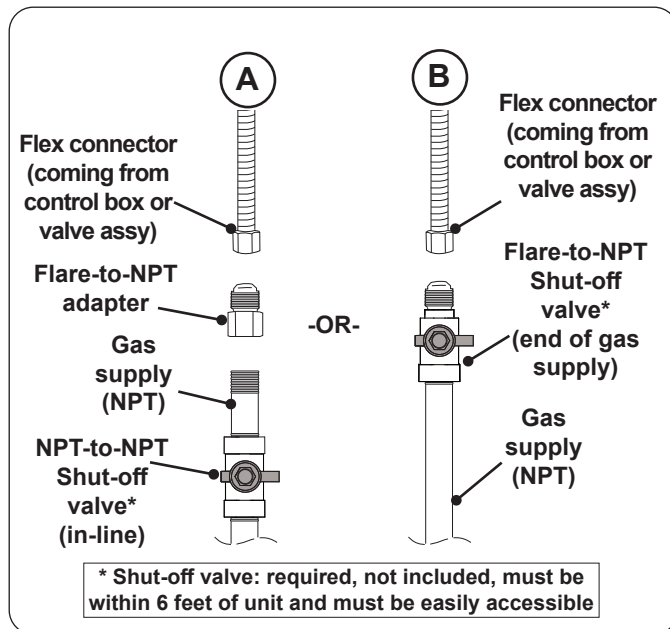
Fig. 29-1 Connecting to a gas line
