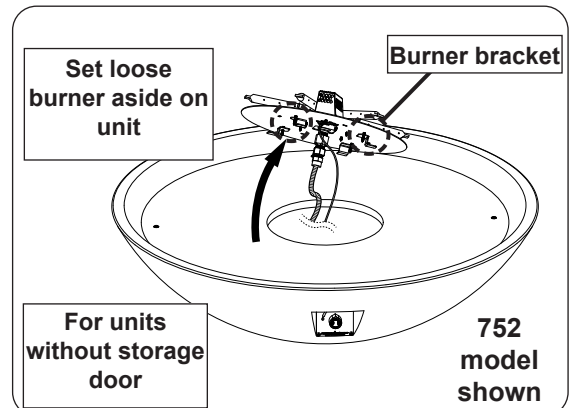
Fig. 26-3 Remove burner assembly (if needed)
