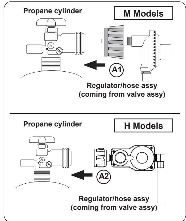
Fig. 28-1 Connecting to an L.P. cylinder
