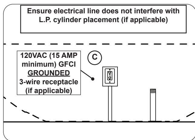
Fig. 24-2 Route electrical (if applicable)
